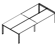
B0814 80x140x74h B1014 100x140x74h B1214 120x140x74h B1414 140x140x74h B1614 160x140x74h B1814 180x140x74h B2014 200x140x74h B2214 220x140x74h bench allineato P140 aligned bench D140
