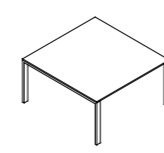
C1414 140x140x74h C1614 160x140x74h C1814 180x140x74h C2014 200x140x74h C2214 220x140x74h tavolo P140 table D140
