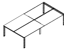
B0816 80x160x74h B1016 100x160x74h B1216 120x160x74h B1416 140x160x74h B1616 160x160x74h B1816 180x160x74h B2016 200x160x74h B2216 220x160x74h bench allineato P160 aligned bench D160
