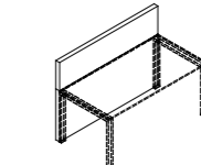
P0812 80x6x120h P1012 100x6x120h P1212 120x6x120h P1412 140x6x120h P1612 160x6x120h P1812 180x6x120h P2012 200x6x120h paretina divisoria H120 partition screen H120
