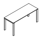
A086 80x60x74h A106 100x60x74h A126 120x60x74h A146 140x60x74h A166 160x60x74h A186 180x60x74h A206 200x60x74h A226 220x60x74h scrivania P60 desk D60
