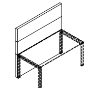
P0816 80x6x160h P1016 100x6x160h P1216 120x6x160h P1416 140x6x160h P1616 160x6x160h P1816 180x6x160h P2016 200x6x160h paretina divisoria H160 partition screen H160
