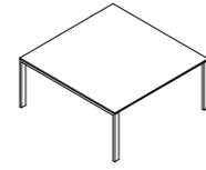
C1616 160x160x74h C1816 180x160x74h C2016 200x160x74h C2216 220x160x74h tavolo P160 table D160
