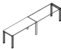
B086 80x60x74h B106 100x60x74h B126 120x60x74h B146 140x60x74h B166 160x60x74h B186 180x60x74h B206 200x60x74h B226 220x60x74h scrivania allineata P60 aligned desk D60
