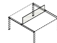
SV0830 80x1x30h SV1030 100x1x30h SV1230 120x1x30h SV1430 140x1x30h SV1630 160x1x30h SV1830 180x1x30h screen in vetro glass screen
