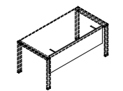
MP0840 80x1,8x40h MP1040 100x1,8x40h MP1240 120x1,8x40h MP1440 140x1,8x40h MP1640 160x1,8x40h MP1840 180x1,8x40h MP2040 200x1,8x40h modesty panel modesty panel
