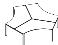
T126 120+120x60x74h T147 140+140x70x74h trifoglio clover
