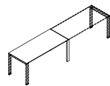
B087 80x70x74h B107 100x70x74h B127 120x70x74h B147 140x70x74h B167 160x70x74h B187 180x70x74h B207 200x70x74h B227 220x70x74h scrivania allineata P70 aligned desk D70
