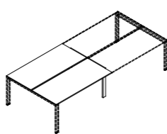
SQB0814 80x140x74h SQB1014 100x140x74h SQB1214 120x140x74h SQB1414 140x140x74h SQB1614 160x140x74h SQB1814 180x140x74h SQB2014 200x140x74h SQB2214 220x140x74h bench allineato P140 aligned bench D140
