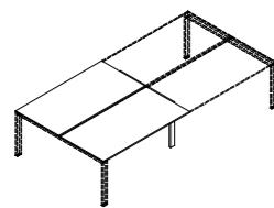
SQB0816 80x160x74h SQB1016 100x160x74h SQB1216 120x160x74h SQB1416 140x160x74h SQB1616 160x160x74h SQB1816 180x160x74h SQB2016 200x160x74h SQB2216 220x160x74h bench allineato P160 aligned bench D160
