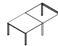
SQD1212 120x120x74h SQD1412 140x120x74h SQD1612 160x120x74h SQD1812 180x120x74h SQD2012 200x120x74h SQD2212 220x120x74h tavolo allineato P120 aligned table D120
