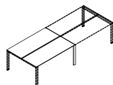
SQB0812 80x120x74h SQB1012 100x120x74h SQB1212 120x120x74h SQB1412 140x120x74h SQB1612 160x120x74h SQB1812 180x120x74h SQB2012 200x120x74h SQB2212 220x120x74h bench allineato P120 aligned bench D120
