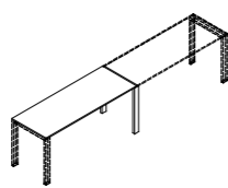
SQB086 80x60x74h SQB106 100x60x74h SQB126 120x60x74h SQB146 140x60x74h SQB166 160x60x74h SQB186 180x60x74h SQB206 200x60x74h SQB226 220x60x74h scrivania allineata P60 aligned desk D60
