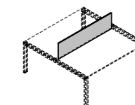
ST0830 80x2x30h ST1030 100x2x30h ST1230 120x2x30h ST1430 140x2x30h ST1630 160x2x30h ST1830 180x2x30h screen in tessuto fabric screen
