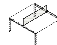
SV0830 80x1x30h SV1030 100x1x30h SV1230 120x1x30h SV1430 140x1x30h SV1630 160x1x30h SV1830 180x1x30h screen in vetro glass screen
