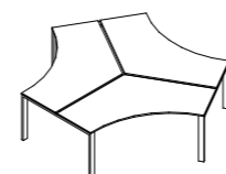
SQT126 120+120x60x74h SQT147 140+140x70x74h trifoglio clover
