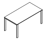
SQA088 80x80x74h SQA108 100x80x74h SQA128 120x80x74h SQA148 140x80x74h SQA168 160x80x74h SQA188 180x80x74h SQA208 200x80x74h SQA228 220x80x74h scrivania P80 desk D80
