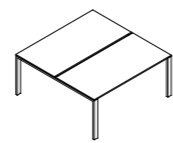
SQA0814 80x140x74h SQA1014 100x140x74h SQA1214 120x140x74h SQA1414 140x140x74h SQA1614 160x140x74h SQA1814 180x140x74h SQA2014 200x140x74h SQA2214 220x140x74h bench P140 bench D140
