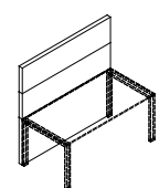
P0816 80x6x160h P1016 100x6x160h P1216 120x6x160h P1416 140x6x160h P1616 160x6x160h P1816 180x6x160h P2016 200x6x160h paretina divisoria H160 partition screen H160
