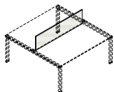
SV0830 80x1x30h SV1030 100x1x30h SV1230 120x1x30h SV1430 140x1x30h SV1630 160x1x30h SV1830 180x1x30h screen in vetro glass screen
