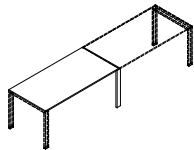
B088 80x80x74h B108 100x80x74h B128 120x80x74h B148 140x80x74h B168 160x80x74h B188 180x80x74h B208 200x80x74h B228 220x80x74h scrivania allineata P80 aligned desk D80
