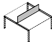
ST0830 80x2x30h ST1030 100x2x30h ST1230 120x2x30h ST1430 140x2x30h ST1630 160x2x30h ST1830 180x2x30h screen in tessuto fabric screen
